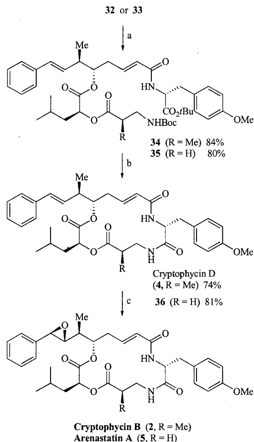
Scheme 4. (a) 2,4,6- \text{Cl}_3\text{C}_6\text{H}_2\text{COCl} , i\text{Pr}_2\text{NEt} , \text{THF} , 23 °C, 2 h, then 25, \text{DMAP} , benzene, 23 °C, 1 h; (b) \text{TFA} , 23 °C, 2 h, then 2,4,6- \text{Cl}_3\text{C}_6\text{H}_2\text{COCl} , i\text{Pr}_2\text{NEt} , \text{DMAP} , \text{THF} , 23 °C, 1 h, then benzene, 23 °C, 12 h; (c) \text{Me}_2\text{C}(\text{O})_2 , \text{CH}_2\text{Cl}_2 , -30 to 23 °C, 12 h
