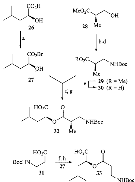
Scheme 3. (a) \text{Cs}_2\text{CO}_3 , \text{MeOH}/\text{H}_2\text{O} (5:1), 23 °C, 30 min, then \text{BnBr} , \text{DMF} , 0 °C, 12 h (quant.); (b) \text{TsCl} , \text{Et}_3\text{N} , \text{CH}_2\text{H}_2 , 0 °C, 1 h (99%); (c) \text{NaN}_3 , \text{DMSO} , 23 °C, 6 h; (d) \text{Boc}_2\text{O} , \text{H}_2 , 10% \text{Pd/C} , \text{EtOAc} , 23 °C, 12 h (quant., 2 steps); (e) \text{LiOH} , \text{EtOH} , 23 °C, 30 min (quant.); (f) \text{DCC} , \text{DMAP} , \text{CH}_2\text{Cl}_2 , 23 °C, 12 h (91%); (g) \text{H}_2 , 5% \text{Pd/C} , \text{EtOAc} , 23 °C, 5 h (95%); (h) \text{H}_2 , 10% \text{Pd/C} , \text{EtOAc} 23 °C, 1 h (97%)
